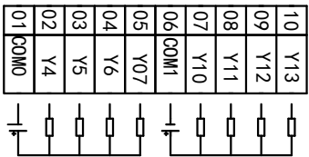
HF_20MR_6MT_MD280_FX_A接线图
